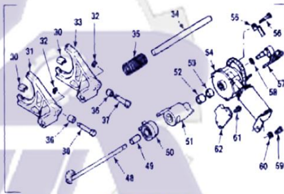
ELECTRIC SHIFT ASSEMBLY
