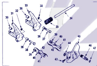
MECHANICAL SHIFT ASSEMBLY
